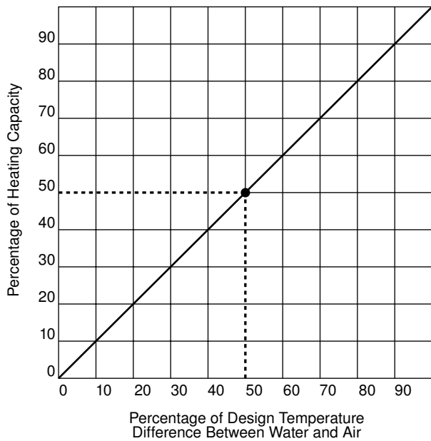
Fig. 4 Controlling heat output by changing water temperatures
