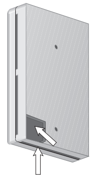
Wiring can enter through the back or the bottom of the enclosure.
